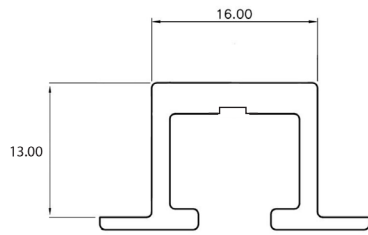
FLUSH FIT TRACK PROFILE
