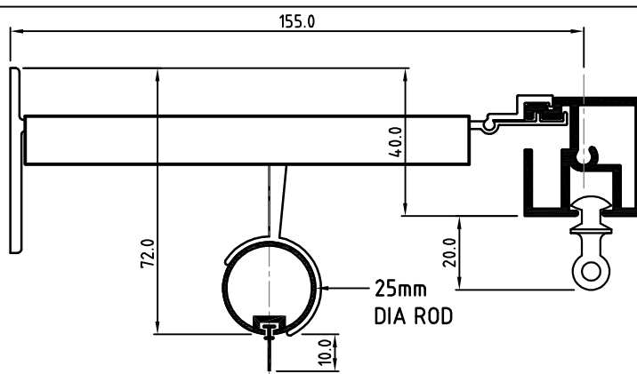
32mm/25mm Glide Bracket
