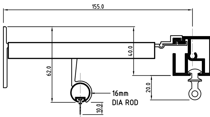
32mm/16mm Glide Bracket
