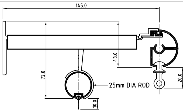
35mm/25mm Glide Bracket
