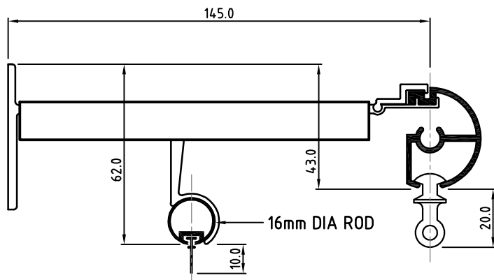
35mm/16mm Glide Bracket
