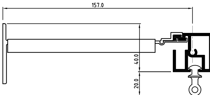
32mm Extended Bracket
