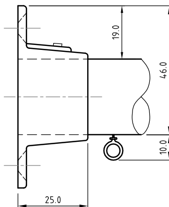
25mm End Wall (Flange) Bracket
