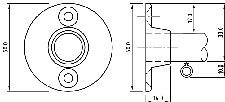
16mm End Wall (Flange) Bracket
